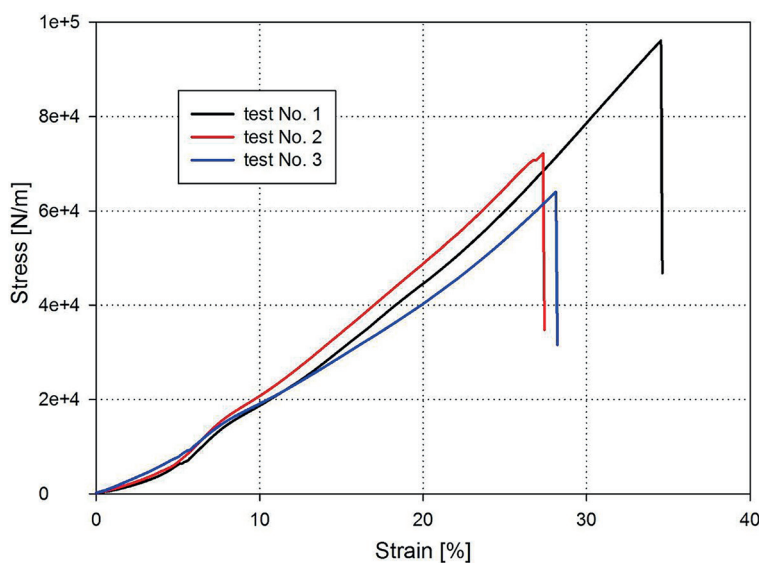
Fig. 5. Experimental strain–stress functions
