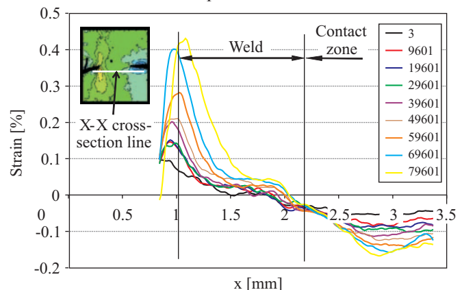
Fig. 21. Strain distribution in u - direction in X-X cross-section, recorded in successive load cycles .
