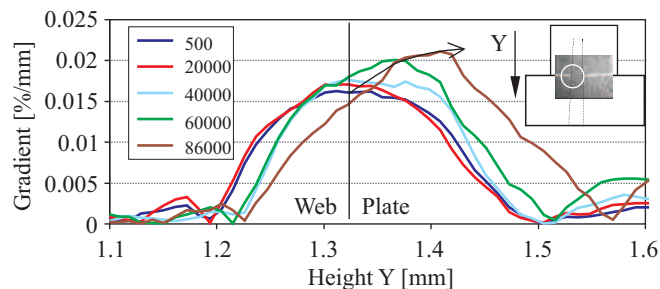
Fig. 17. Gradients of \varepsilon_{uv} strain .
