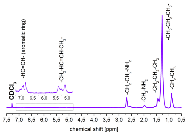
Fig. 5 1 H NMR spectrum of bio-based diamine PRIAMINE 1071
