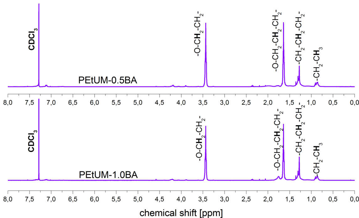
Fig. 6 1 H NMR spectra of selected poly(ether-urethane-urea)s i.e. PEtUM-0.5BA and PEtUM-1.0BA
