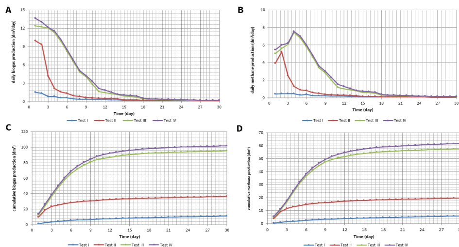
Figure 3. Daily production of: (a) biogas; (b) methane and accumulation curves of: (c) biogas; (d) methane production.
