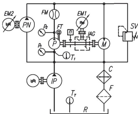
Fig. 5. The diagram of the measurement system of the test stand [27]: P – tested pump, M – hydraulic motor, PN – pump for fill the leaks in P and M, IP – impeller pump (pre-supply pump), SV – safety valve, C – cooler, F – filter, R – reservoir, IAG – intersecting axis gear, EM1 and EM2 – electric motors with frequency converters, other designations – description in the text below
