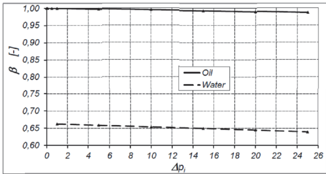
Fig.10. Degree of laminarity of the flow \beta in flat clearances of the pump for oil and water [25]
