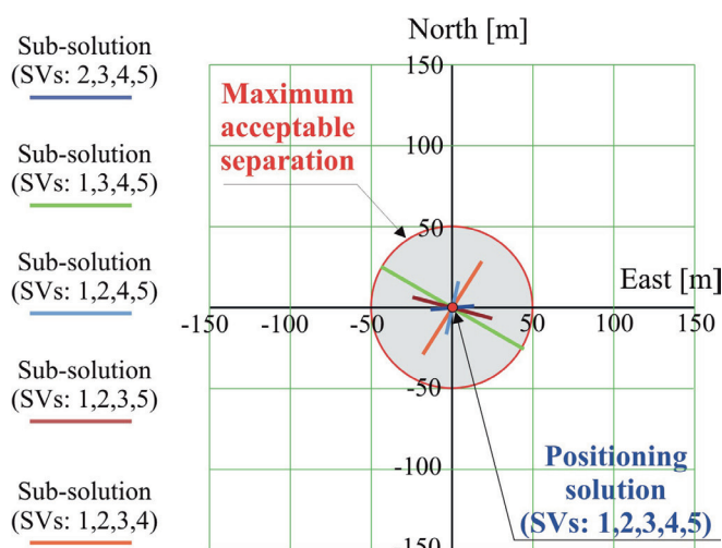
Fig. 4. Obtained sub-solutions distribution related to the positioning solution if there are no outliers in pseudorange measurements
