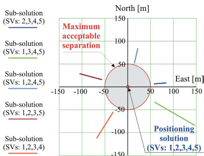
Fig. 5. Obtained sub-solutions distribution related to the positioning solution if outlier equal 200 m appeared in pseudorange measurement to SV1
