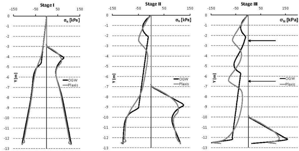
Fig. 11. Soil pressure acting on the sheet pile wall with struts.
