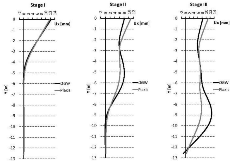
Fig. 10. Horizontal displacements of the sheet pile wall with struts.
