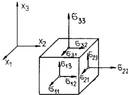
FIGURE 5. Presentation of stress state components [11].
