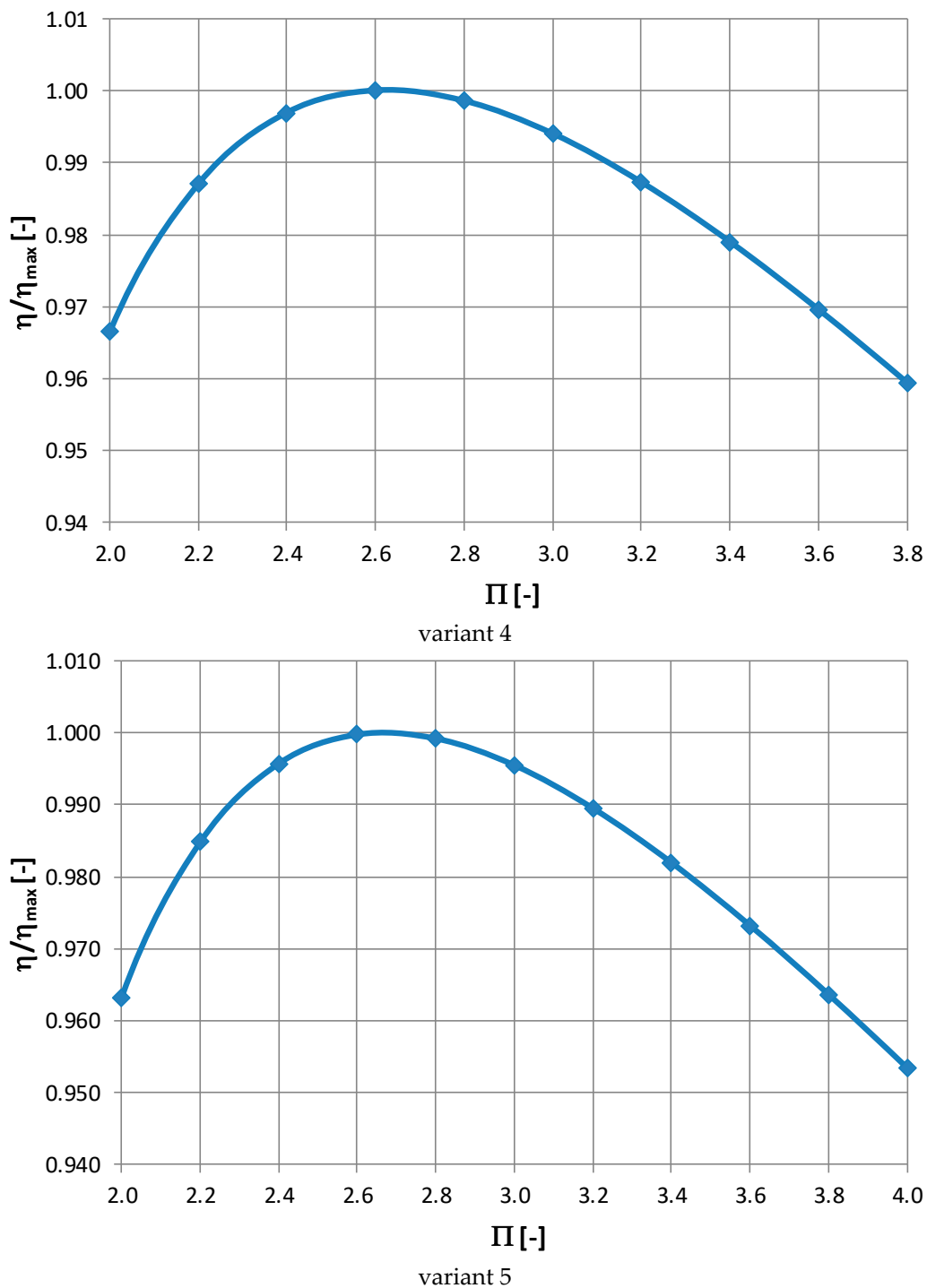
Figure 4. The influence of pressure ratio on the efficiency of the analyzed variants of turbine sets.
