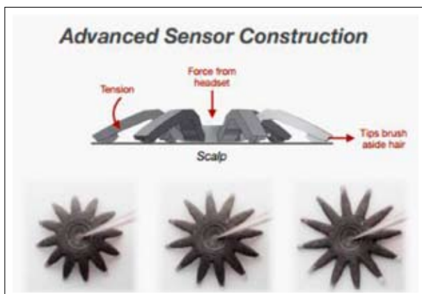
Fig. 1. Flexible dry EEG electrode made by Cognionics
