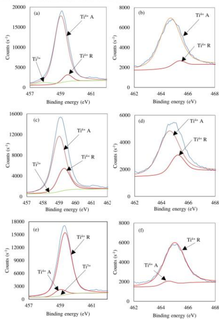
Figure 18. Deconvolution of X-ray photoelectron spectroscopy (XPS) spectra for Ti 2p 3/2 and 2p 1/2 for TBT-HIO 3 _20_300 (a,b), TBT-HIO 3 _20_400 (c,d) and TBT-HIO 3 _20_450 (e,f).
