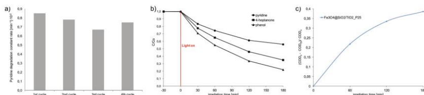
Fig. 8. Pyridine degradation constant rate in the presence of \text{Fe}_3\text{O}_4/\text{SiO}_2/\text{TiO}_2 .P25 measured in the fourth subsequent cycles (a), Photocatalytic decomposition of aqueous solution of three model pollutants using \text{Fe}_3\text{O}_4/\text{SiO}_2/\text{TiO}_2 .P25 nanocomposite (b) Degradation of organic compounds from flow back water. The COD removal as a function of time for \text{Fe}_3\text{O}_4/\text{SiO}_2/\text{TiO}_2 .P25 photocatalyst (c).
