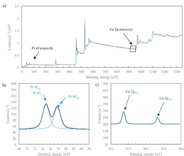
Figure 5. XPS spectra for d- \text{TiO}_2 -20-Pt0.1/Cu0.1 sample (a) with the deconvolution for Pt 4f (b) and Cu 2p (c).
