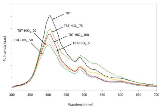
Figure 10. Photoluminescence (PL) spectra for defective \text{TiO}_2 -HfO 2 samples.
