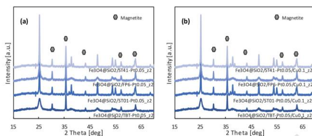
Fig. 1. XRD patterns of mono-metal (a) and bi-metal (b) \text{Fe}_3\text{O}_4@ \text{SiO}_2/\text{TiO}_2\text{-M} magnetic photocatalysts
