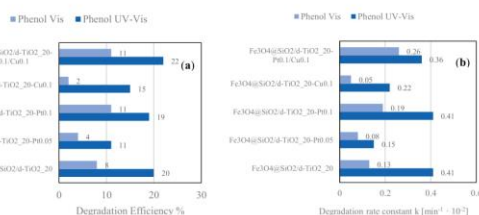
Figure 8. Efficiency of phenol degradation in UV-Vis and Vis light for magnetic \text{Fe}_3\text{O}_4/\text{SiO}_2/\text{d-TiO}_2\text{-Pt/Cu} photocatalysts, presented as % of degradation (a) and rate constant k (b).
