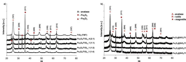
Fig. 2. XRD patterns of \text{Fe}_3\text{O}_4/\text{TiO}_2 nanoparticles (a); \text{Fe}_3\text{O}_4/\text{SiO}_2/\text{TiO}_2 nanocomposites varying the source of \text{TiO}_2 NPs (b).
