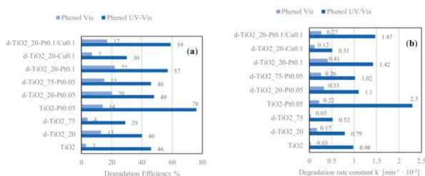
Figure 7. Efficiency of phenol degradation in UV-Vis and Vis light for d-TiO 2 -Pt/Cu photocatalysts, presented as % of degradation (a) and rate constant k (b).
