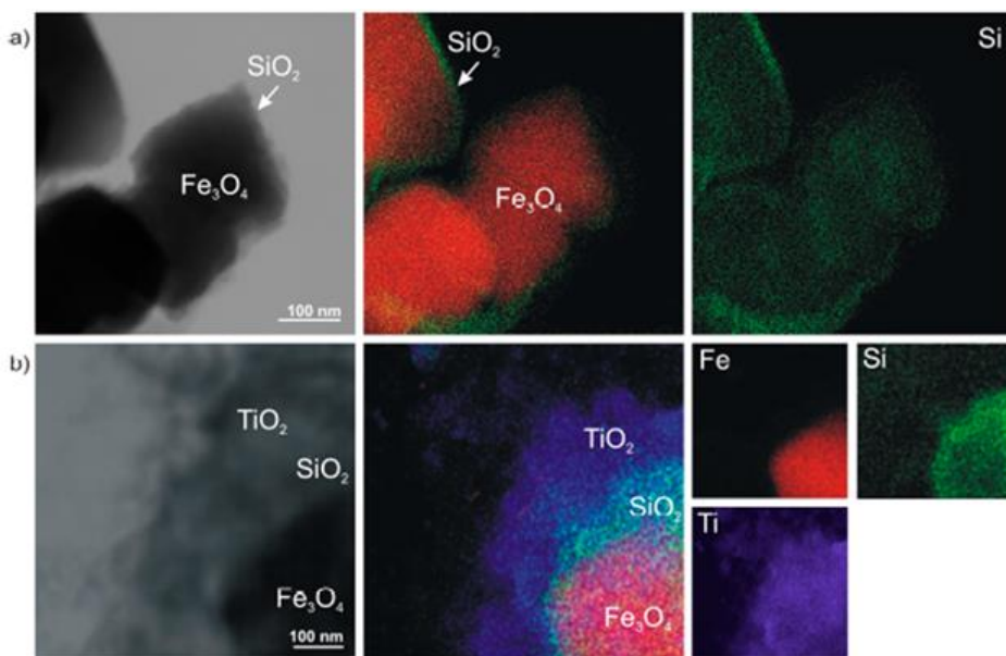
Figure 14. STEM images of \text{Fe}_3\text{O}_4@\text{SiO}_2 (a) and \text{Fe}_3\text{O}_4@\text{SiO}_2/\text{TiO}_2 (b) combined with mappings of Ti, Fe and Si elements [P5].
