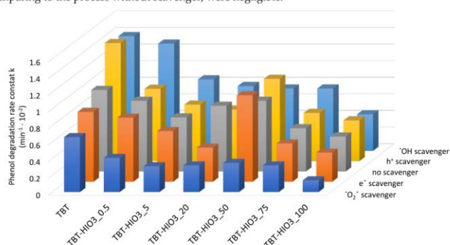
Figure 14. UV-Vis photocatalytic degradation of phenol for TiO 2 -HIO 3 photocatalyst in the presence of \text{e}^- , \text{h}^+ , \cdot\text{O}_2^- , and \cdot\text{OH} scavengers.
