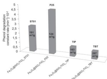
Fig. 7. Degradation constant rates of \text{Fe}_3\text{O}_4/\text{SiO}_2/\text{TiO}_2 nanoparticles prepared using different \text{TiO}_2 matrix.
