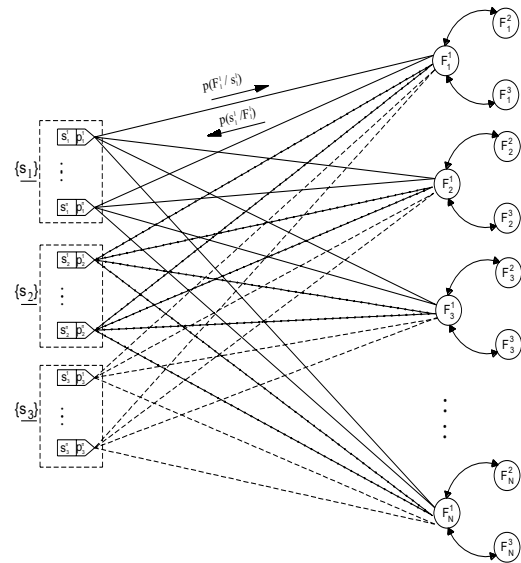
Fig.3. Topological diagnostic model of measurement
