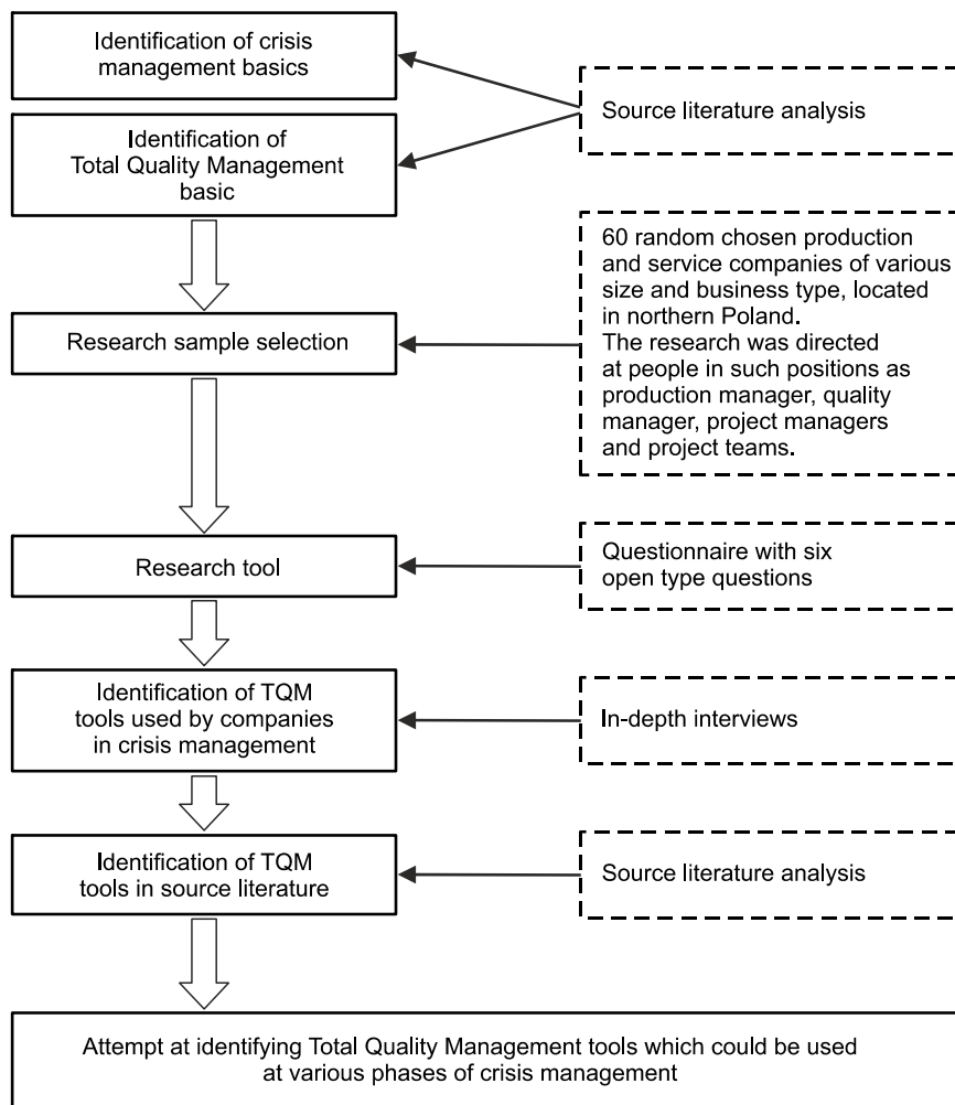
Figure 2. Research methodology
