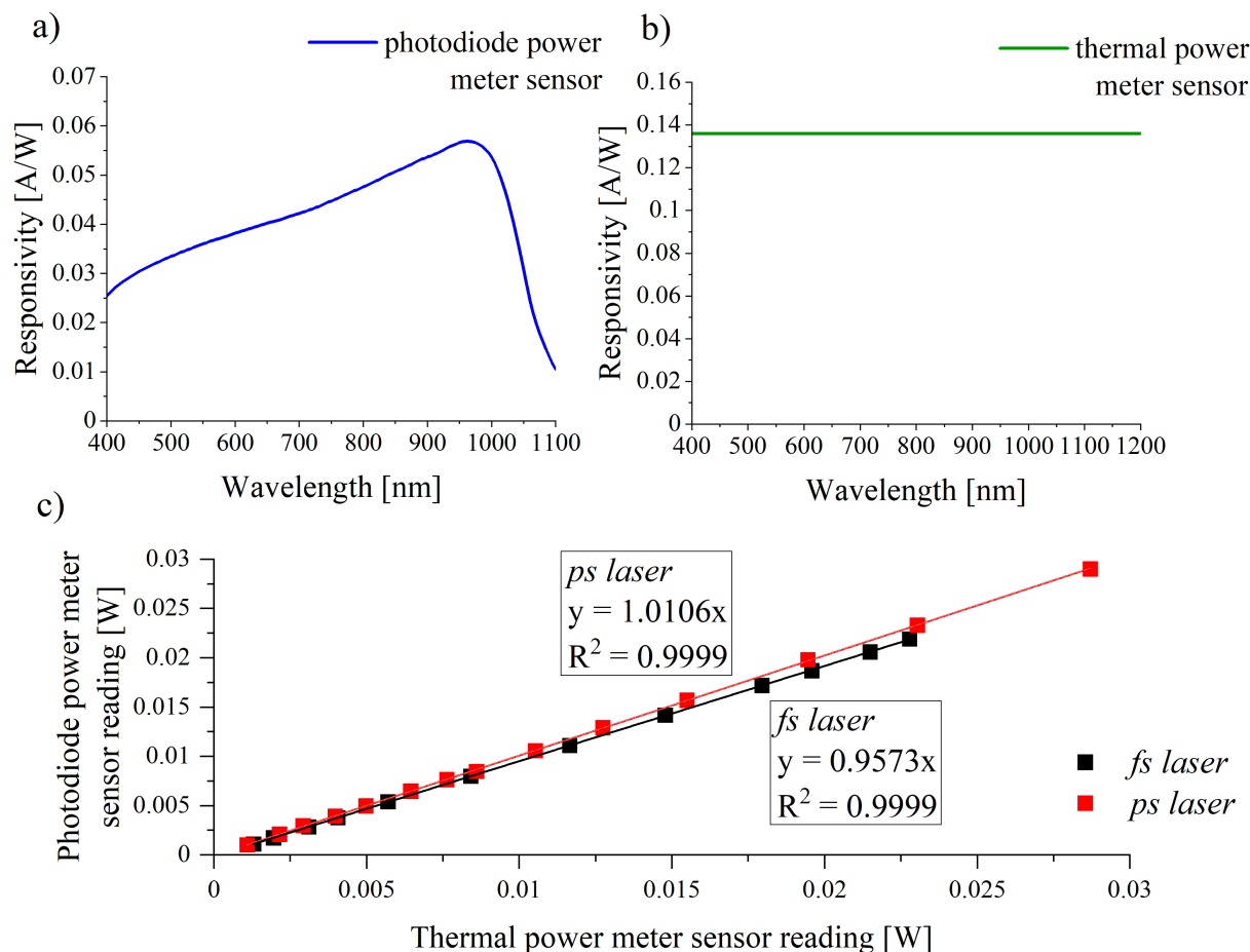
Fig. 8-9. Power level measurement uncertainty. a) Spectral characteristics of photodiode power meter sensor (S120C, Thorlabs). b) Spectral characteristics of thermal power meter sensor (S401C, Thorlabs). c) Differences in power meter sensors readings for both lasers. Solid lines represent a linear fit of the data. The slope coefficients of the fitting lines correspond to the difference between the real and measured power levels.
