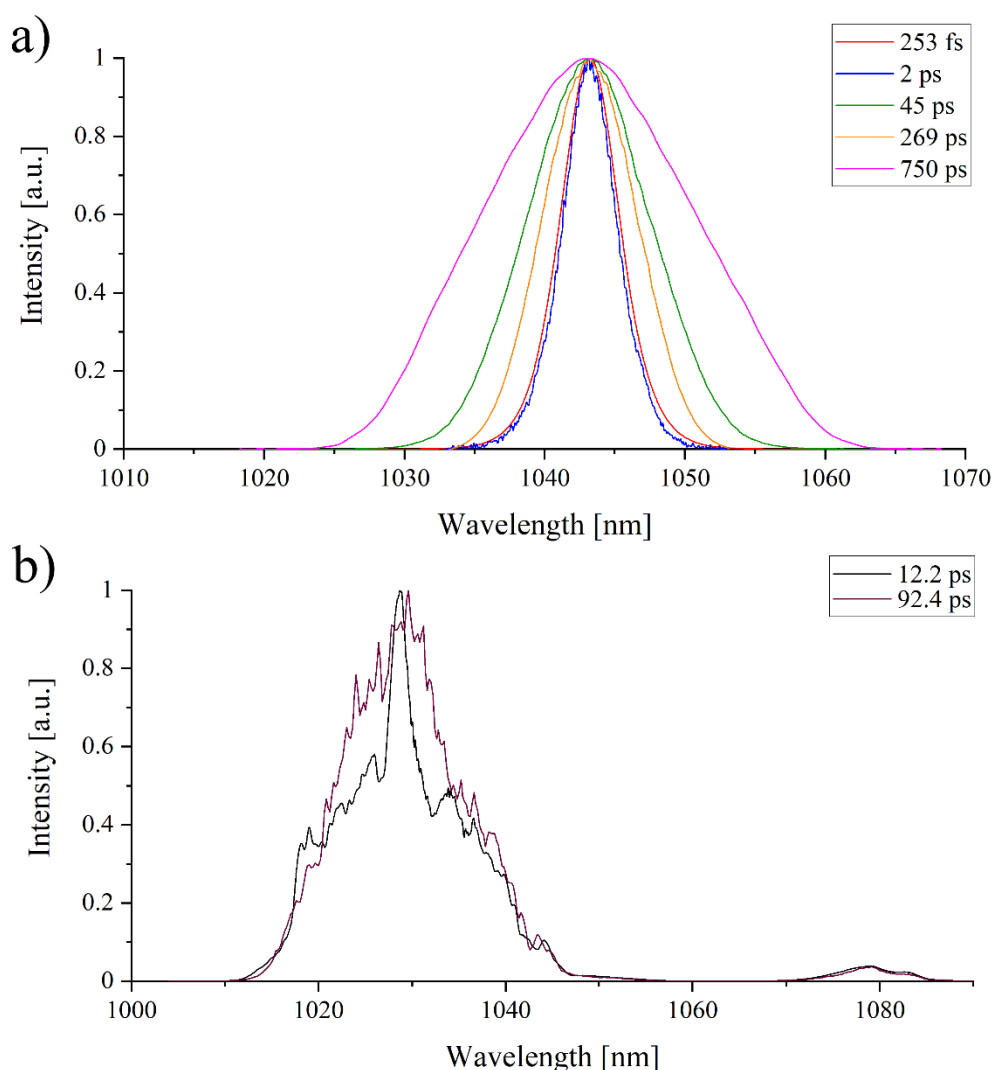
Fig. 7-9. Spectral properties of laser pulse trains originated from: a) fs laser , b) ps laser . The pulse repetition rate is equal to 62.65 MHz and 19.17 MHz for a) and b), respectively. All plots are normalized to 1.
