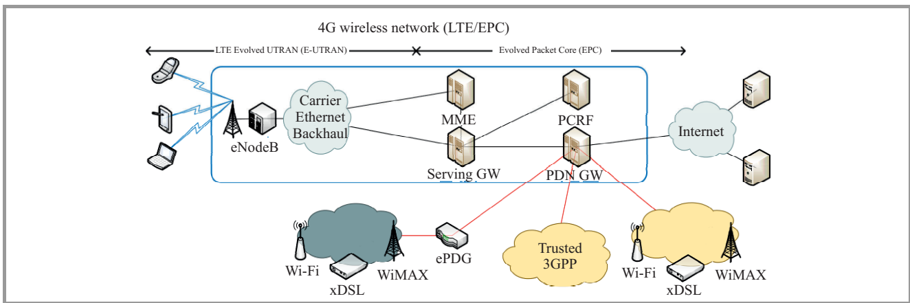
Fig. 11. 4G (LTE Advanced) network architecture.
