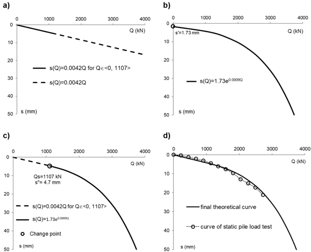
Figure 8: Stages of Q–s characteristics prediction based on the proposed procedure: (a) linear elastic stage; (b) non-linear elastic stage; (c) combination of the linear elastic stage for Q \in \langle 0, Q_s \rangle and non-linear elastic stage; (d) comparison of the theoretical curve with the measured curve from static load test.
