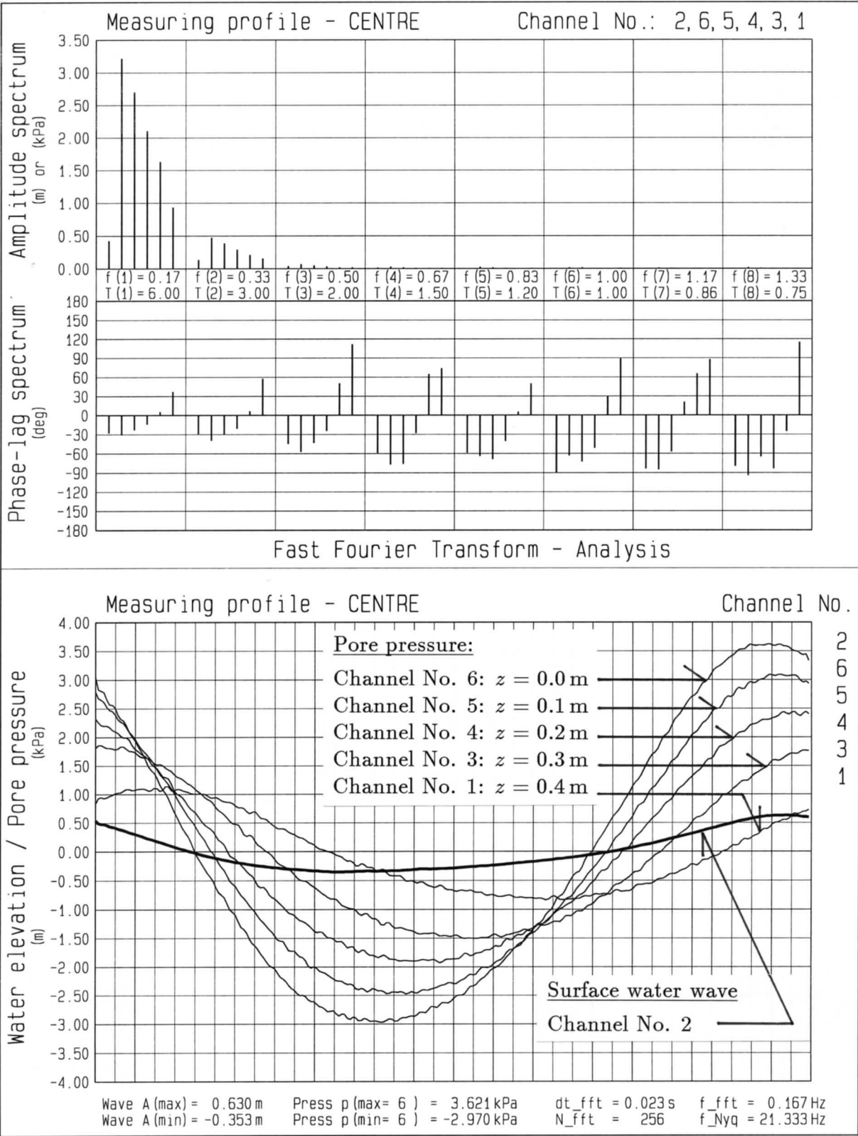
Figure 5.8 Example of graphical presentation of GWK-data analysis (FFT-analysis and plot of recorded signals; Test No. GWK-23, H = 1.0\text{ m} , T = 6\text{ s} , h = 4.5\text{ m} )
