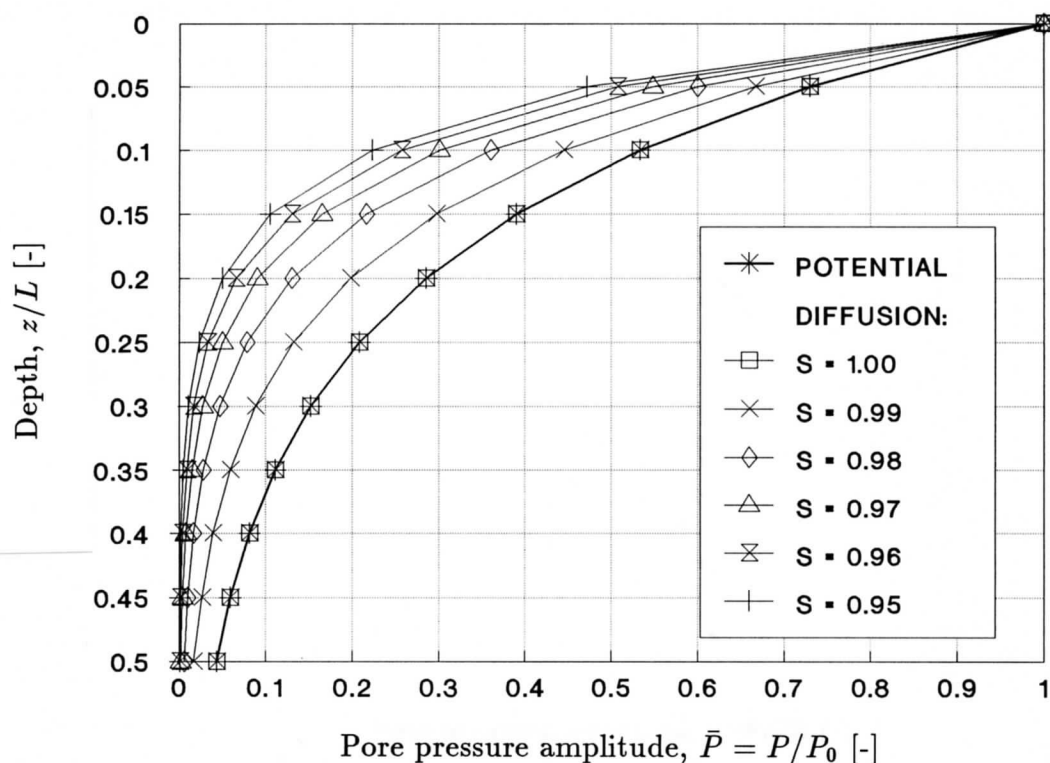
Figure 4.6 Wave-induced pore pressure amplitude distribution with depth in permeable seabed layer of infinite thickness, and for different soil saturation conditions (diffusion problem; k = 10^{-2} m/s)
