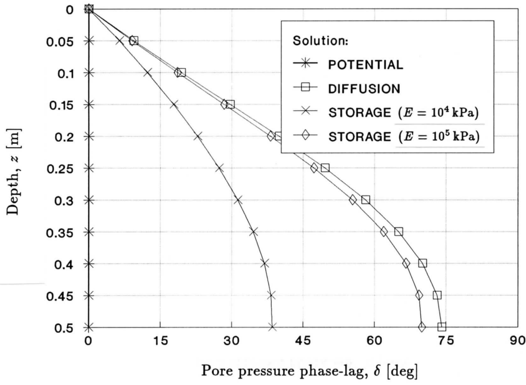
Figure 4.18 Wave-induced pore pressure phase-lag distribution with depth (‘finite-thickness layer’ analytical solution) – comparison between the potential, diffusion ( S = 0.95 ), and storage ( S = 0.95 , E = 10^5 kPa – dense sandy sediments, and E = 10^4 kPa – loose sandy sediments) solutions
