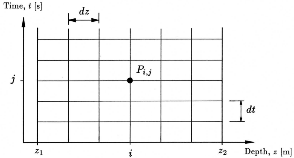
Figure 4.24 Rectangular mesh used in Finite Difference Methods [Jankowski, 1983]
