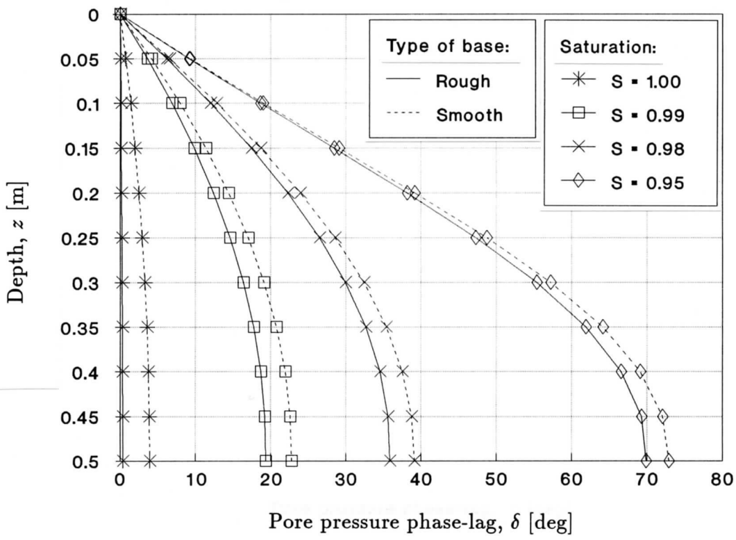
Figure 4.22 Wave-induced pore pressure phase-lag distribution with depth, for different soil saturation conditions and types of impermeable base (2-D storage problem – ‘finite-thickness layer’ analytical solution; E = 10^4 kPa – loose sandy sediments)
