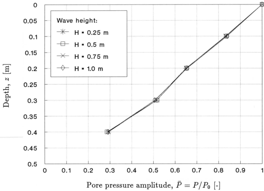
Figure 5.11 Pore pressure amplitude distribution with depth (GWK-tests with constant wave period, T = 6 s)
