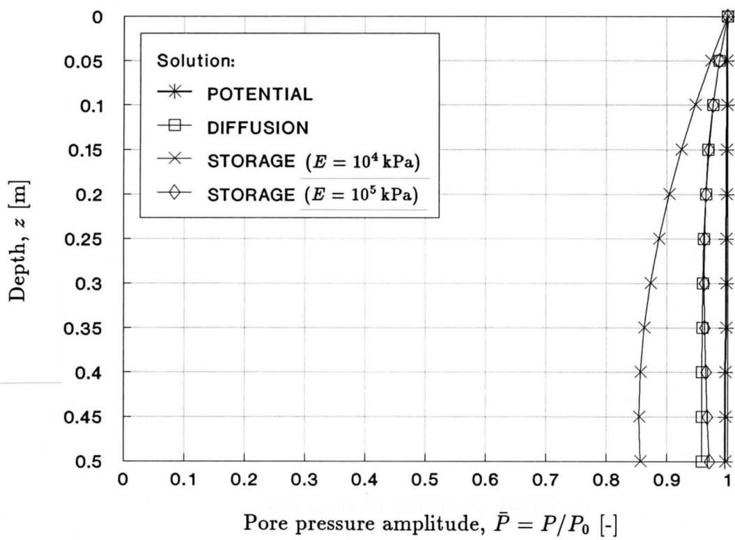
Figure 4.15 Wave-induced pore pressure amplitude distribution with depth (‘finite-thickness layer’ analytical solution) – comparison between the potential, diffusion ( S = 0.99 ), and storage ( S = 0.99 , E = 10^5 kPa – dense sandy sediments, and E = 10^4 kPa – loose sandy sediments) solutions
