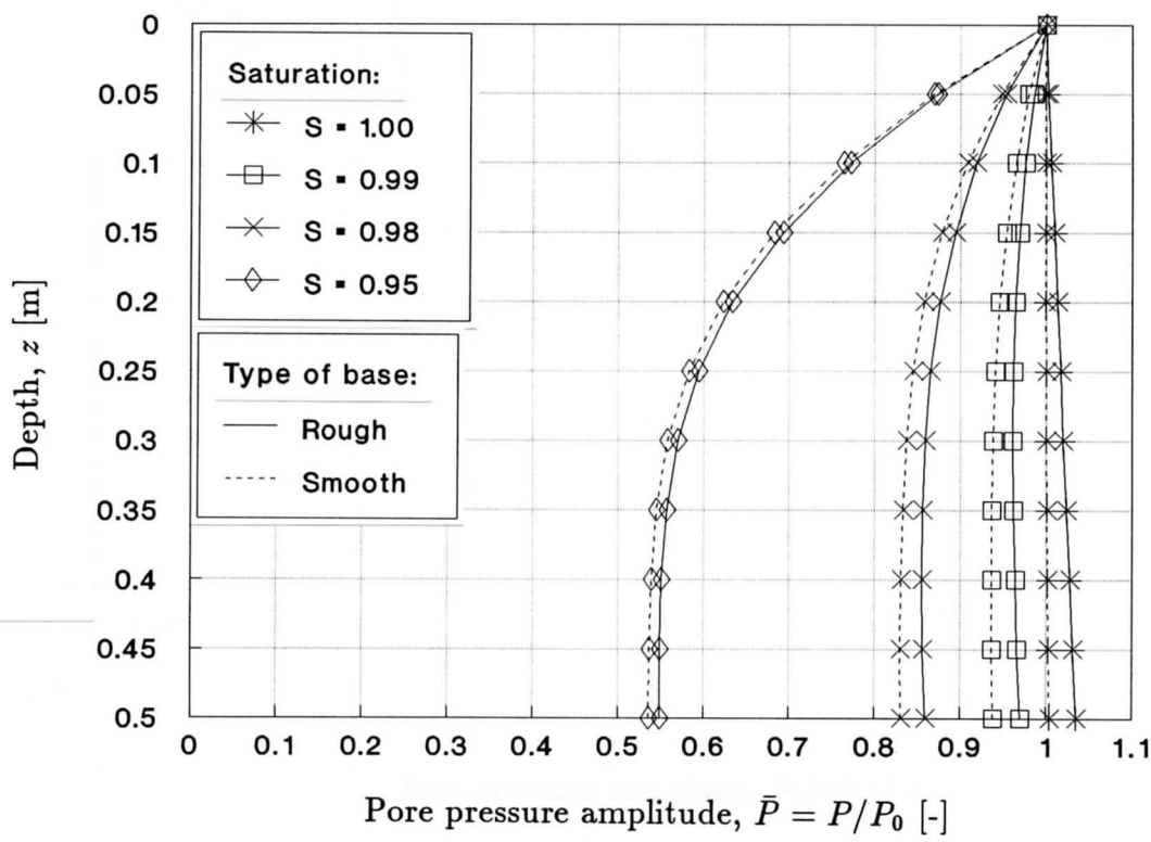
Figure 4.21 Wave-induced pore pressure amplitude distribution with depth, for different soil saturation conditions and types of impermeable base (2-D storage problem – ‘finite-thickness layer’ analytical solution; E = 10^4 kPa – loose sandy sediments)
