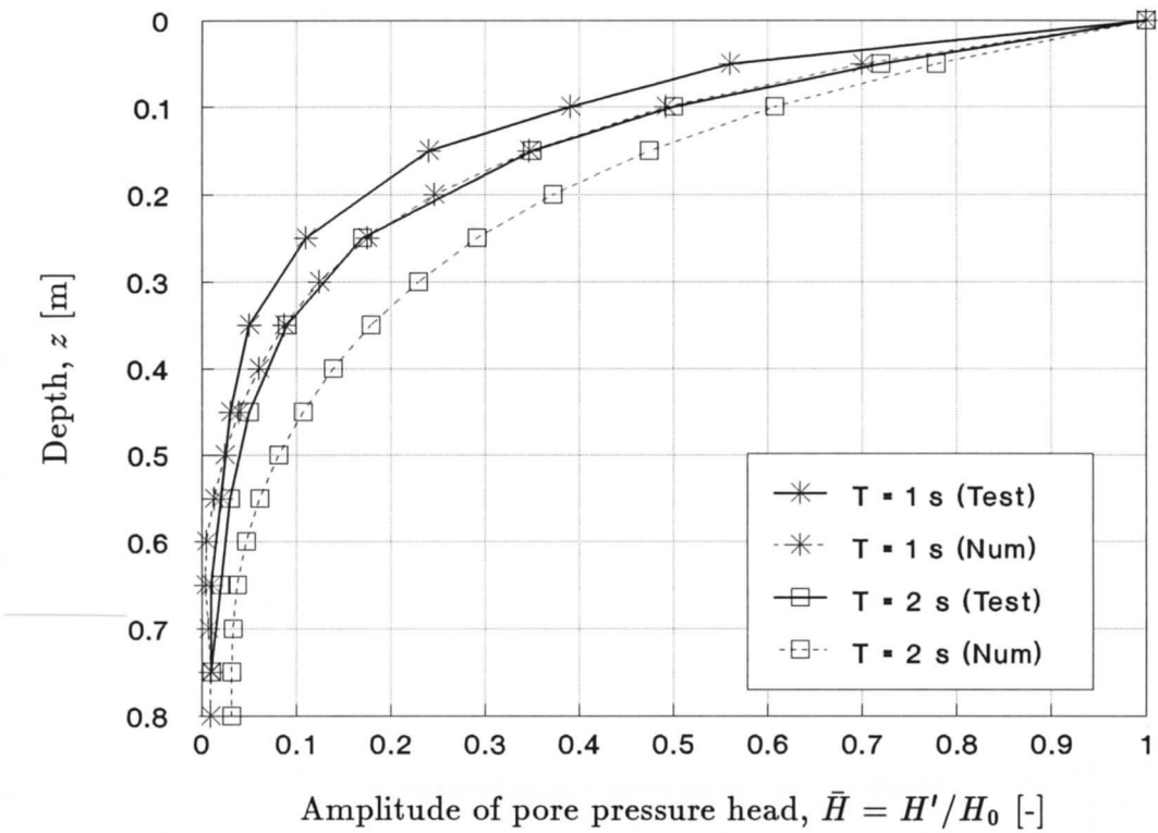
Figure 5.28 Distribution of the amplitude of pore pressure head with depth in the sand column; measurement (Test) versus numerical solution (Num) to 1-D storage problem [Sand G30T, S = 0.830 ]
