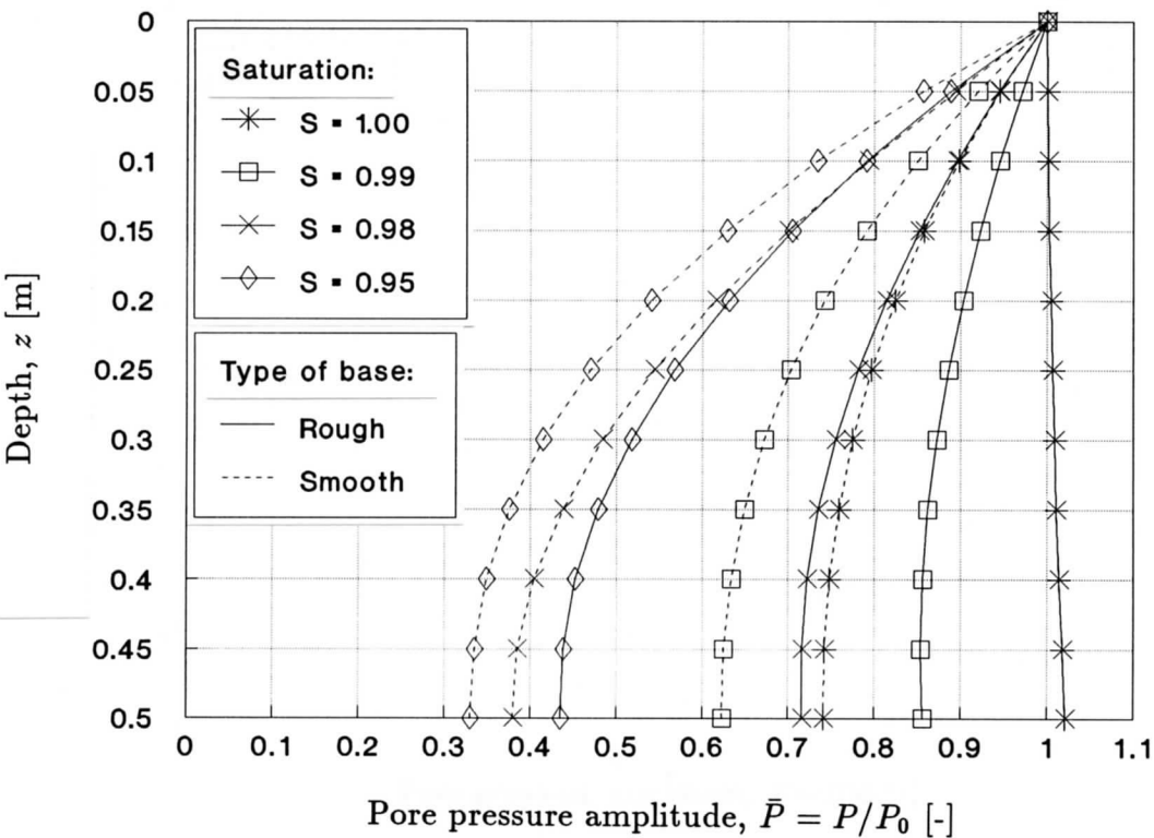
Figure 4.19 Wave-induced pore pressure amplitude distribution with depth, for different soil saturation conditions and types of impermeable base (2-D storage problem – ‘finite-thickness layer’ analytical solution; E = 10^5 kPa – dense sandy sediments)
