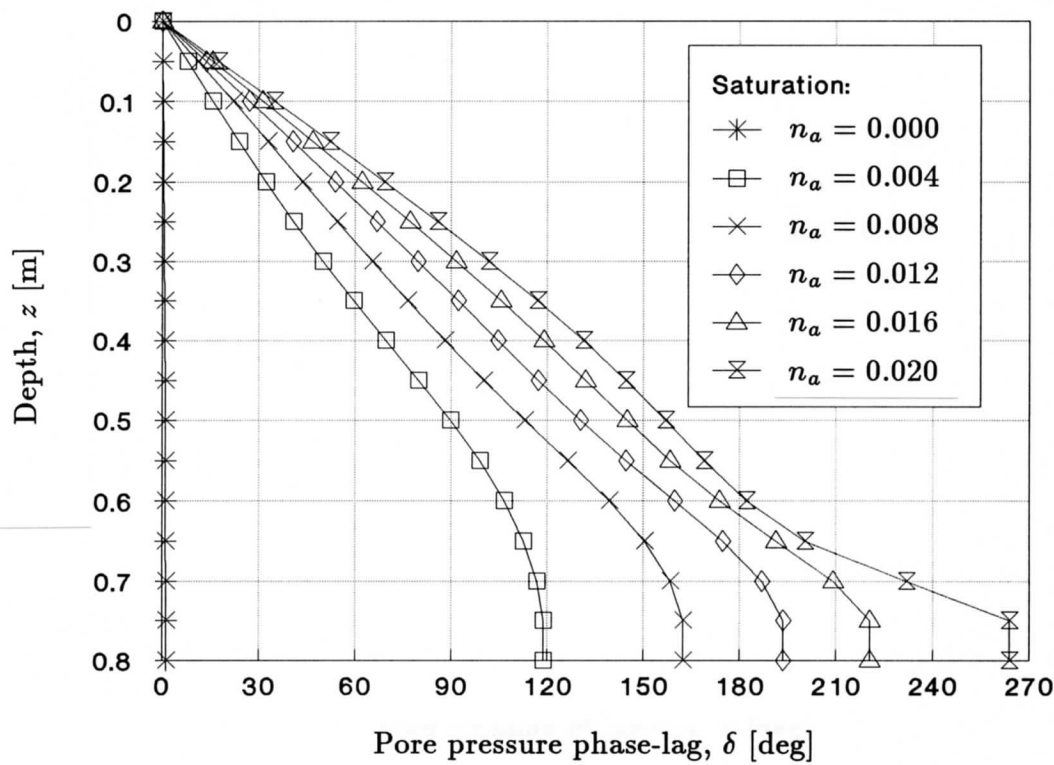
Figure 4.30 Distribution of the pore pressure phase-lag with depth, for different soil saturation conditions and near-incompressible soil (1-D storage model; \alpha_z = 10^{-7} \text{ m}^2/\text{kN} )
