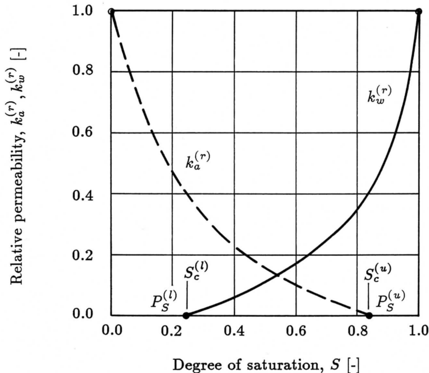
Figure 3.6 Relative permeability to air and water of three-phase sand versus degree of saturation [Keřdi, 1974]
