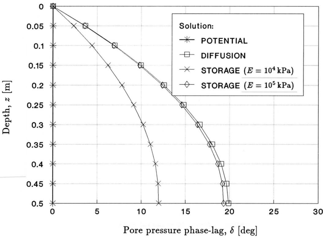
Figure 4.16 Wave-induced pore pressure phase-lag distribution with depth (‘finite-thickness layer’ analytical solution) – comparison between the potential, diffusion ( S = 0.99 ), and storage ( S = 0.99 , E = 10^5 kPa – dense sandy sediments, and E = 10^4 kPa – loose sandy sediments) solutions
