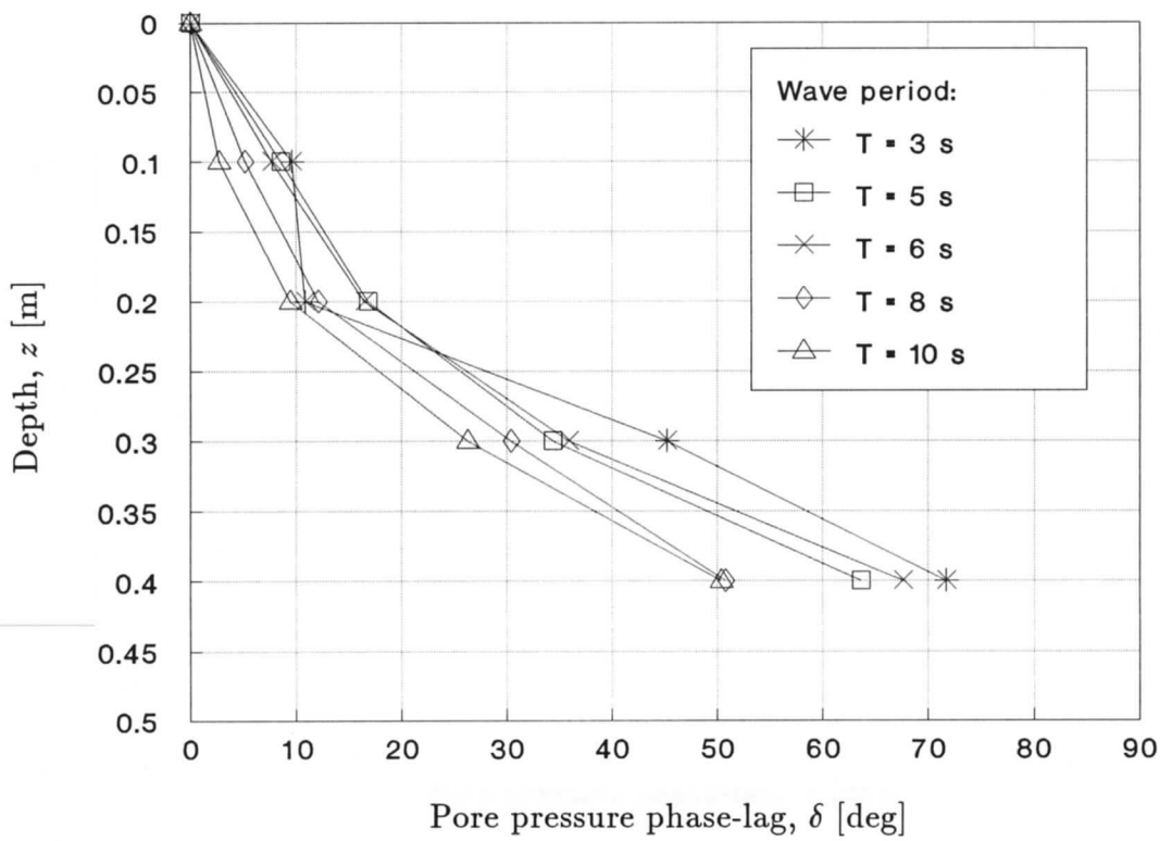
Figure 5.10 Pore pressure phase-lag distribution with depth (tests with constant wave height, H = 1.0 m)
