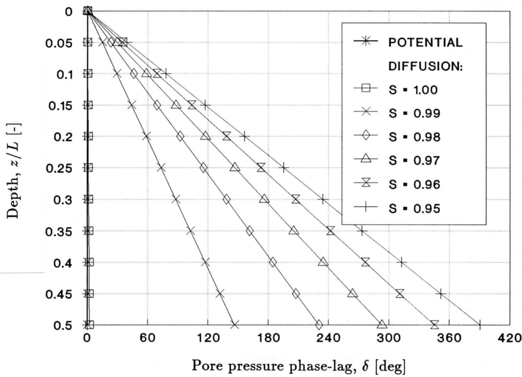
Figure 4.7 Wave-induced pore pressure phase-lag distribution with depth in permeable seabed layer of infinite thickness, and for different soil saturation conditions (diffusion problem; k = 10^{-2} m/s)
