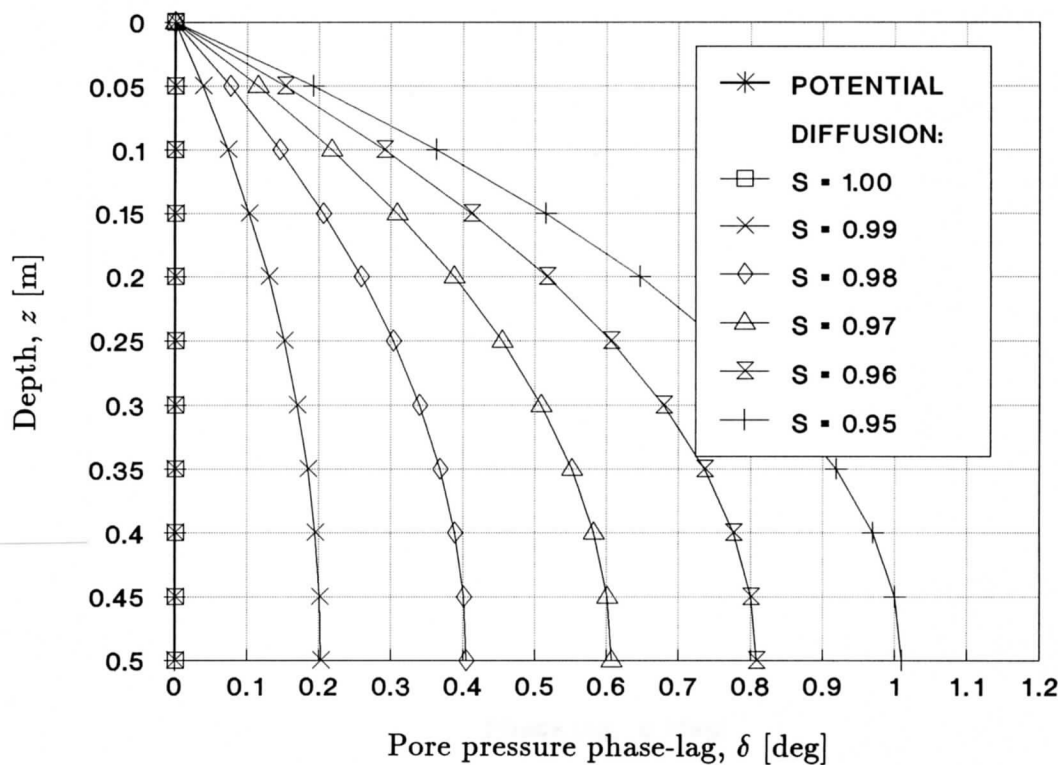
Figure 4.12 Wave-induced pore pressure phase-lag distribution with depth in permeable seabed layer of finite thickness, and for different soil saturation conditions (diffusion problem; k = 10^{-2} m/s)
