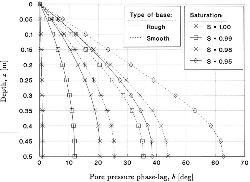
Figure 4.20 Wave-induced pore pressure phase-lag distribution with depth, for different soil saturation conditions and types of impermeable base (2-D storage problem – ‘finite-thickness layer’ analytical solution; E = 10^5 kPa – dense sandy sediments)
