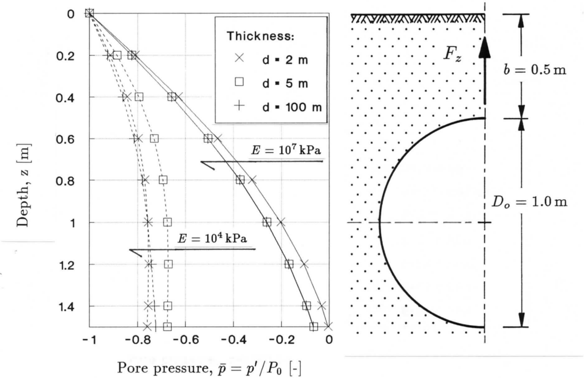
Figure 6.8 Definition sketch for the hydrodynamic uplift force analysis (pore pressure gradient influenced by soil skeleton compressibility and seabed layer thickness; degree of saturation S = 0.99 )
