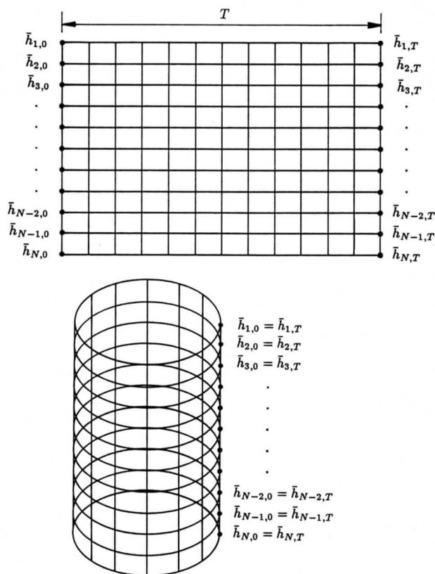
Figure 4.27 Rectangular mesh used in numerical computations with a repeatable and harmonic water loading induced on the top of one-dimensional sand column numerical model
