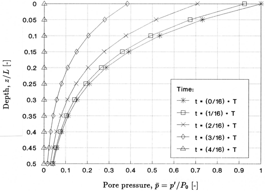
Figure 4.3 Wave-induced pore pressure distribution with depth in permeable seabed layer of infinite thickness, computed for different phases of wave loading cycle (potential problem)
