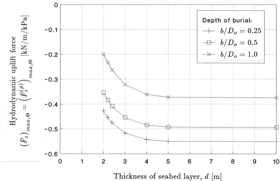
Figure 6.6 Influence of seabed layer thickness and depth of burial on the hydrodynamic uplift force (potential model)
