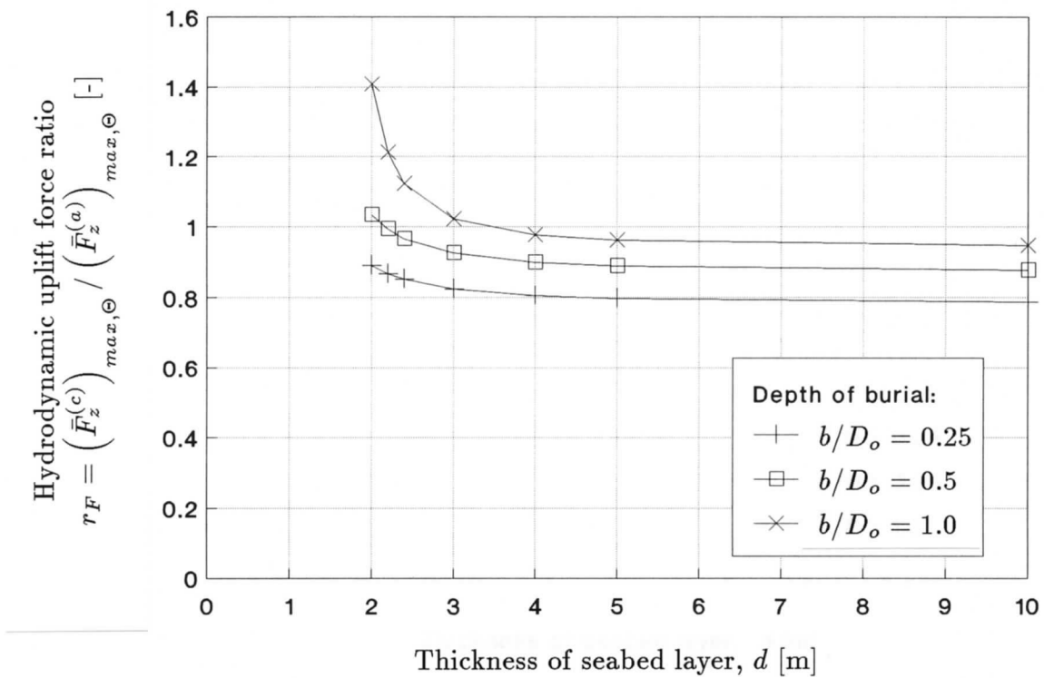
Figure 6.7 Influence of seabed layer thickness and depth of burial on the hydrodynamic uplift force ratio (potential model)
