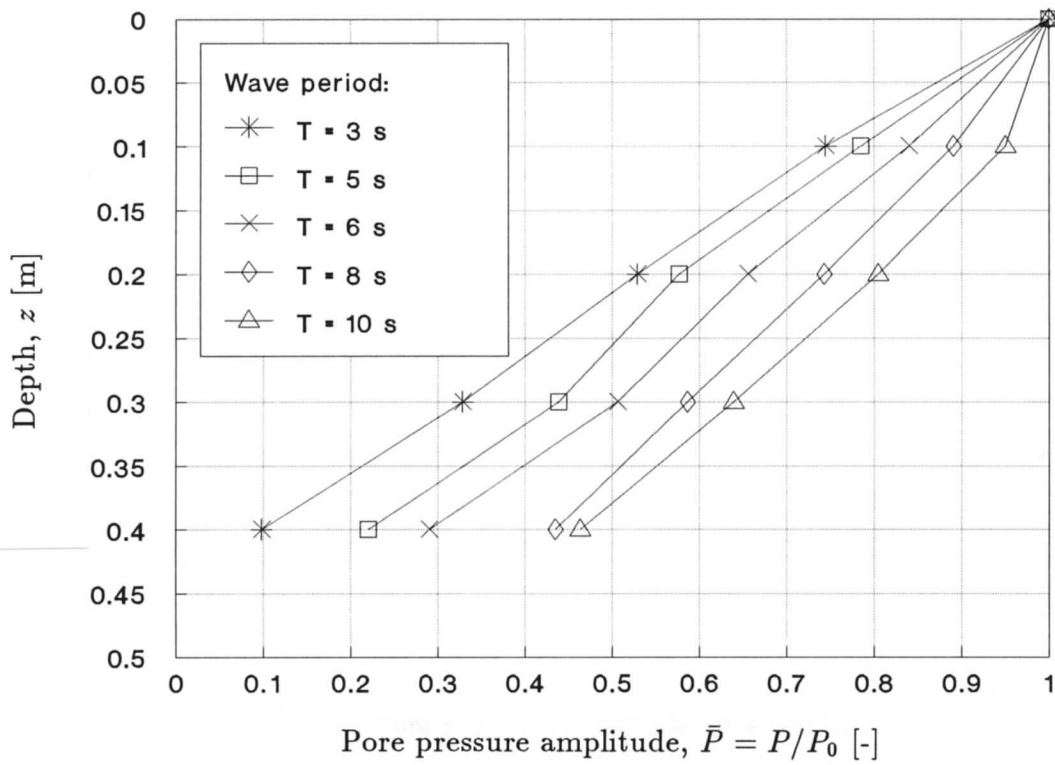
Figure 5.9 Pore pressure amplitude distribution with depth (tests with constant wave height, H = 1.0 m)
