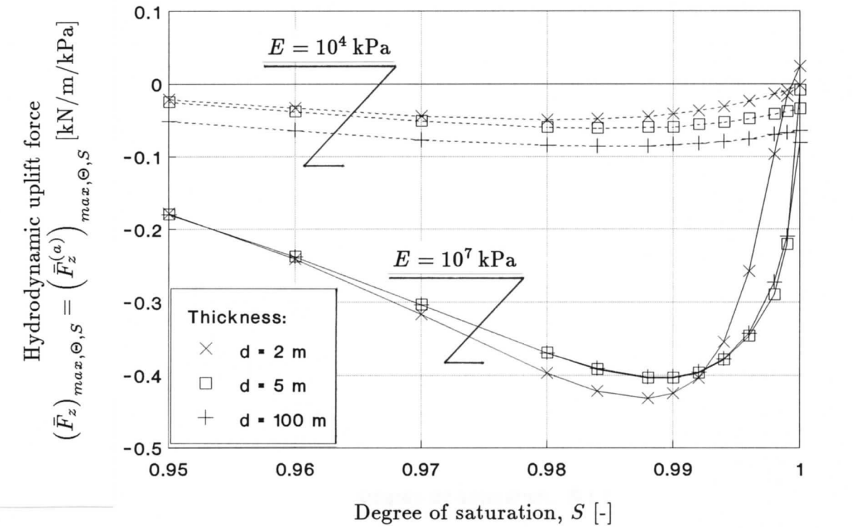
Figure 6.9 Hydrodynamic uplift force versus different soil saturation conditions and compressibility (represented by Young's modulus, E ) of soil skeleton
