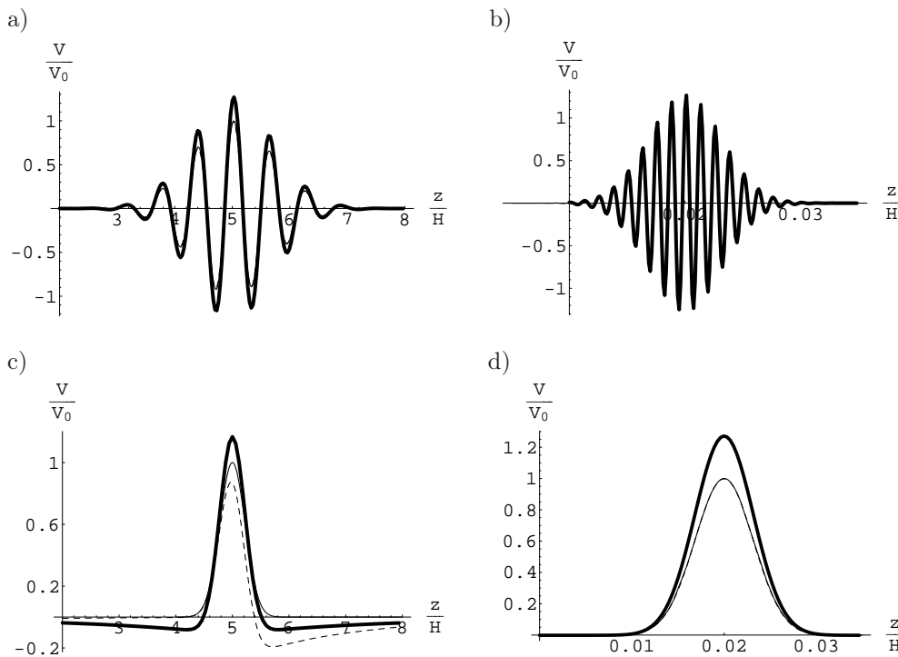
Fig. 1. The waveform V/V_0 as a function of vertical distance z/H (solid line), \frac{1}{\pi V_0} \int_{-\infty}^{\infty} dz' F(z' - z) \frac{\partial V(z')}{\partial z'} (bold line), \frac{1}{V_0} \exp(-z/2H) \int_{-\infty}^z dz' \exp(z'/2H) \frac{\partial V(z')}{\partial z'} (dotted line). At the sets a, b, and d, the dotted and solid curves are very close to each other.
