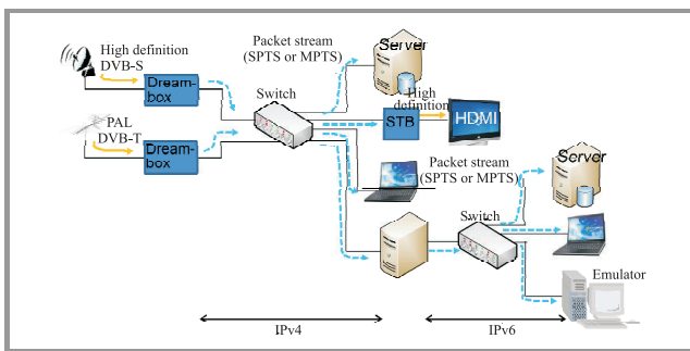
Fig. 4. The IPTV system in IPv4/IPv6 environment. PAL (phase alternating line), DVB-S (digital video broadcasting-satellite), DVB-T (digital video broadcasting-terrestrial), HDMI (high definition multimedia interface), STB (set top box), SPRS (single program transport stream), MPTS (multiple program transport stream).
