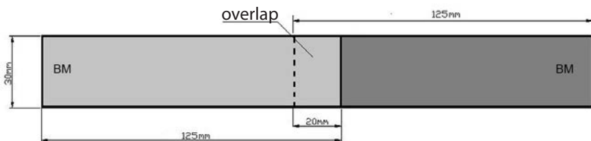
Fig. 1. Schematic overlay brazed joints, BM – base material
